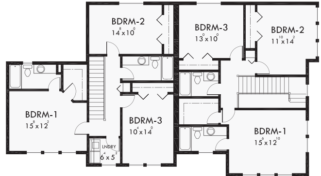
UPPER FLOOR
