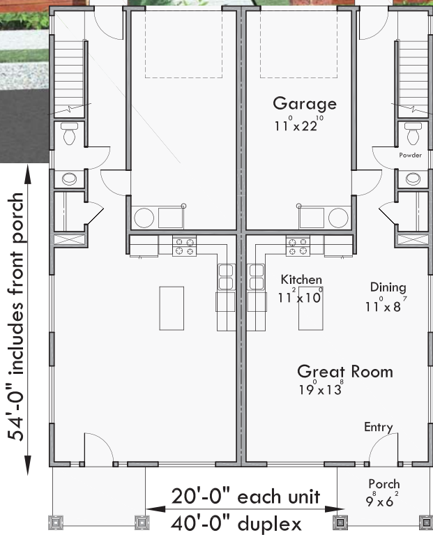
MAIN FLOOR
